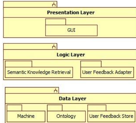
Figure 3: UML Class Diagram – Layer View
