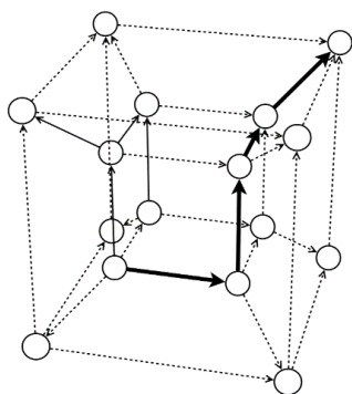
Figure 1: 4D Hypercube
