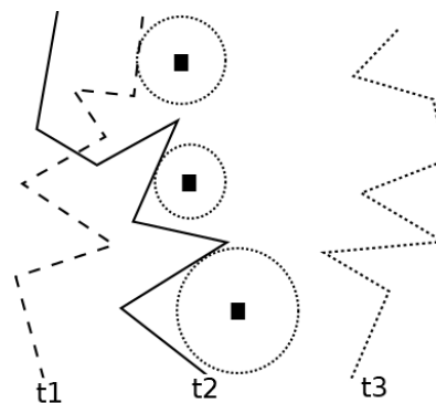
Figure 2: IkNN-Query
